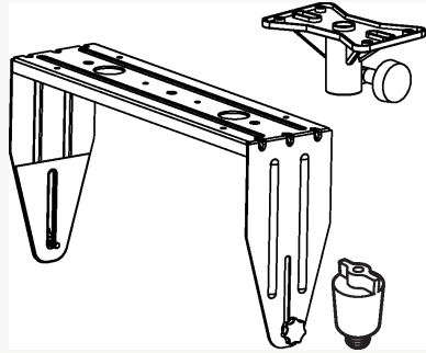
MYA-X40 Yoke
