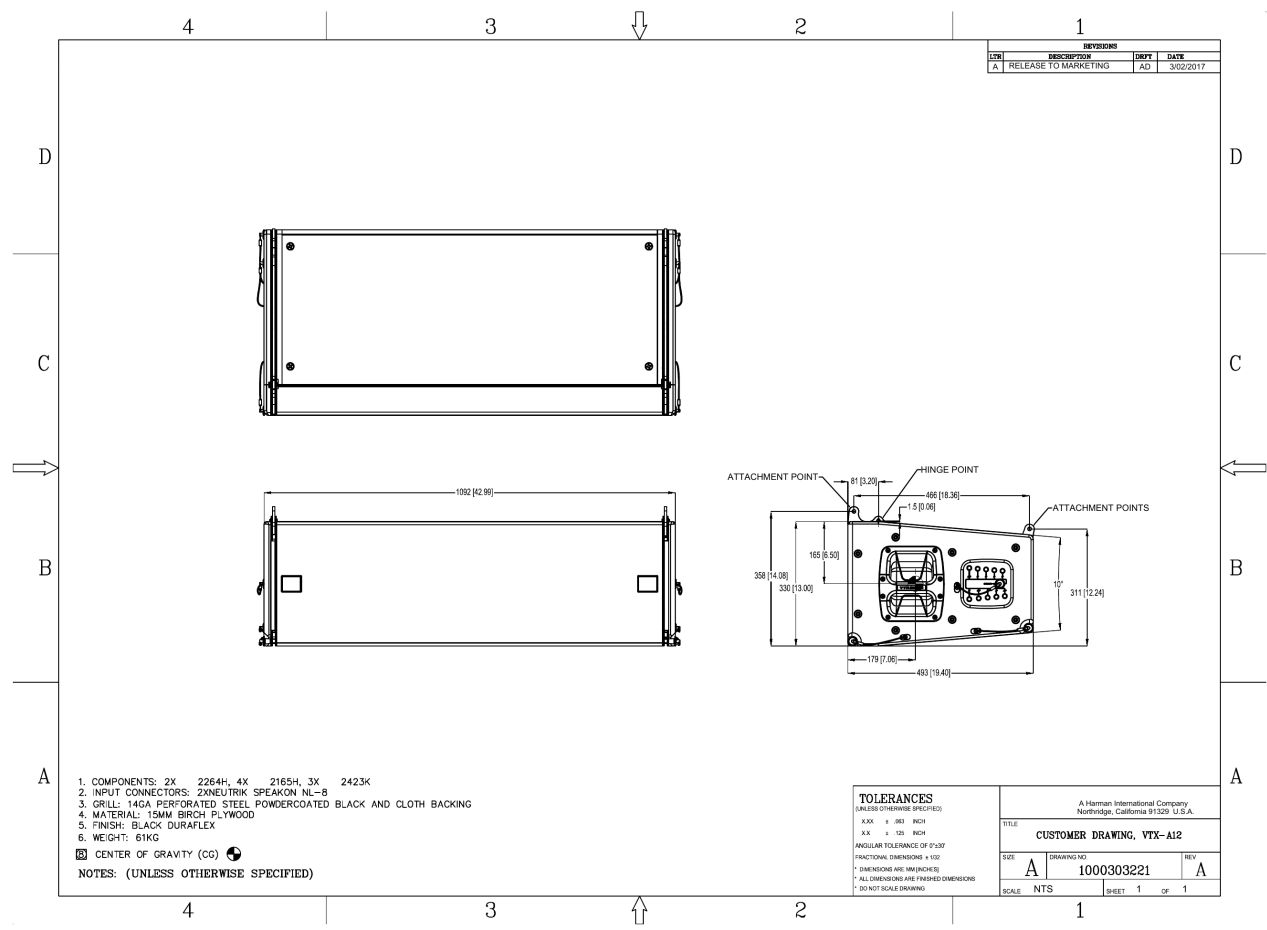
Official customer drawing: 330 mm × 1118 mm × 495 mm / 13 in × 44 in × 19.5 in (H × W × D)
